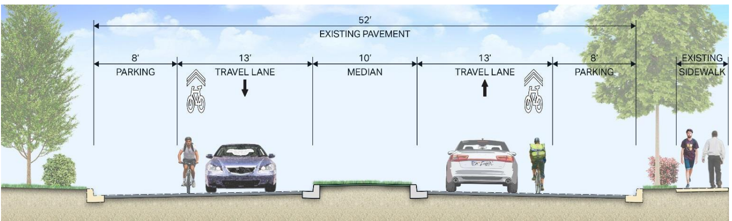
Typical Section with 10' Median
